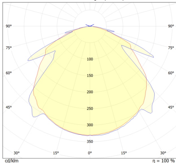
Photometry: (120°)
